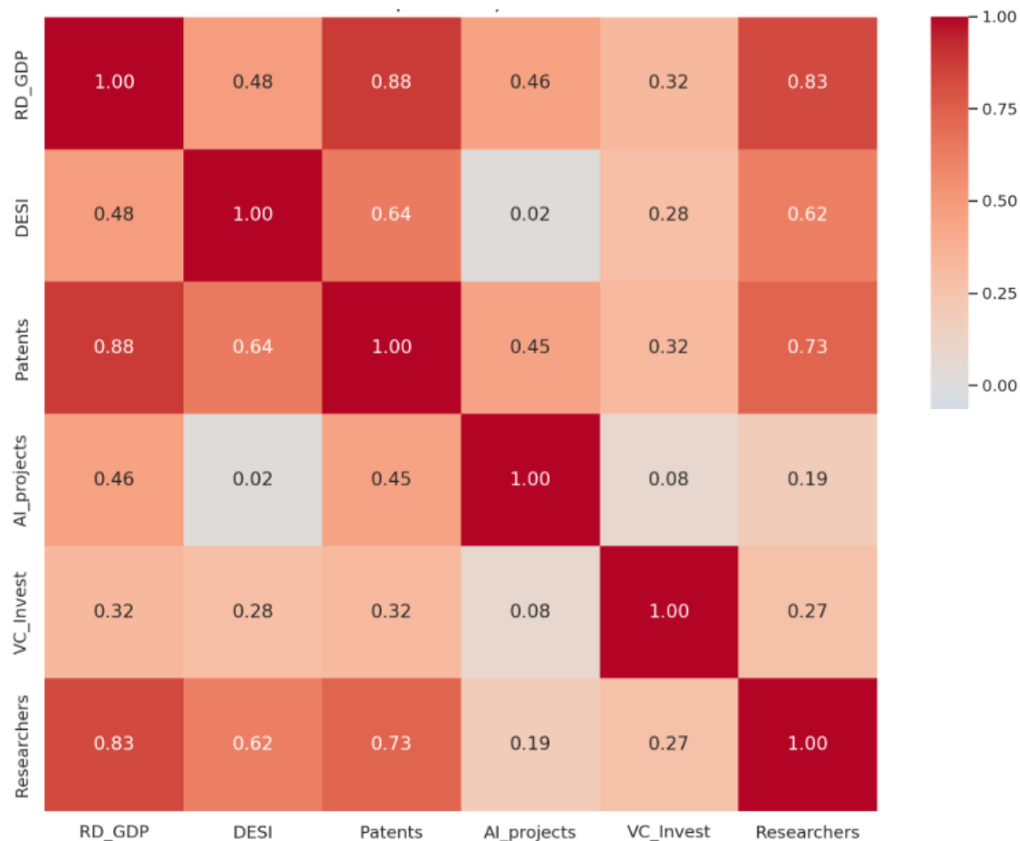
Figure 3. Correlation outputs_heatmap_2017, Reference: authors' elaboration.
