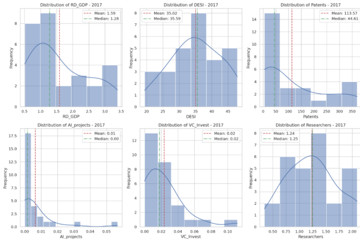
Figure 5. Histograms of Variables – 2017, Reference: authors' elaboration.
