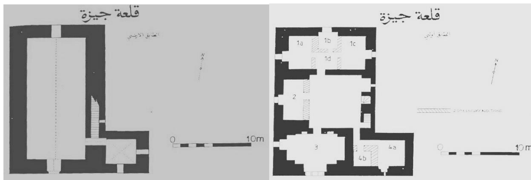
Figure 2: Jizah fort plan. Ground floor; first floor.(Petersen, 2001)
